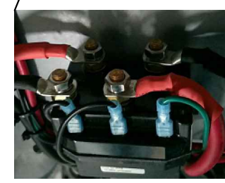
Reversing Contactor
