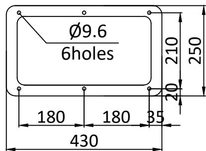
View A
